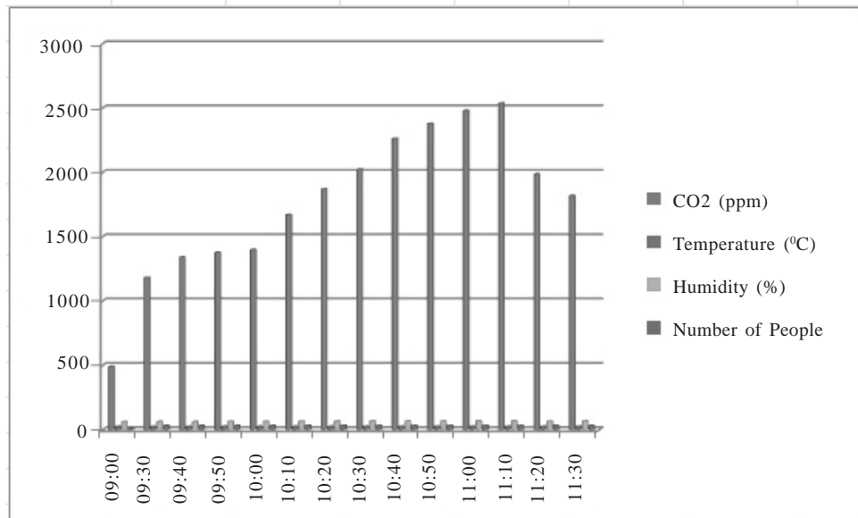
Fig. 3. The amount of CO2 of Lyscnam
